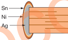
Figure 1 Termination Code T
