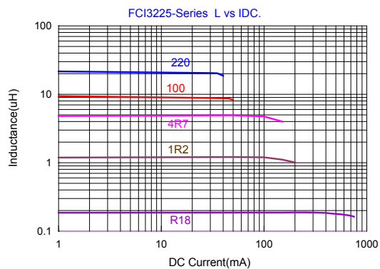
■ Inductance-Current
