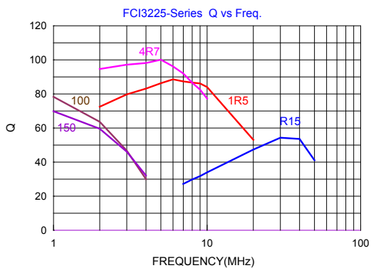
■ Q-Frequency Characteristics
